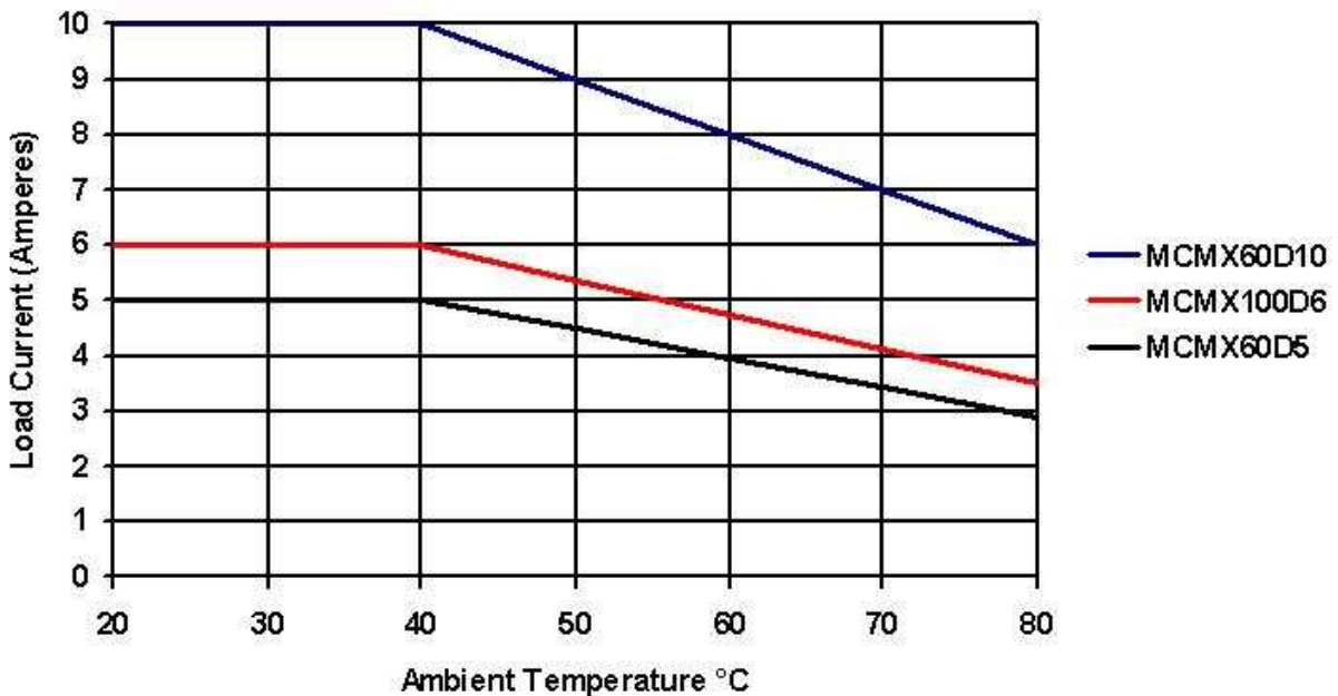
Current Derating Curves
