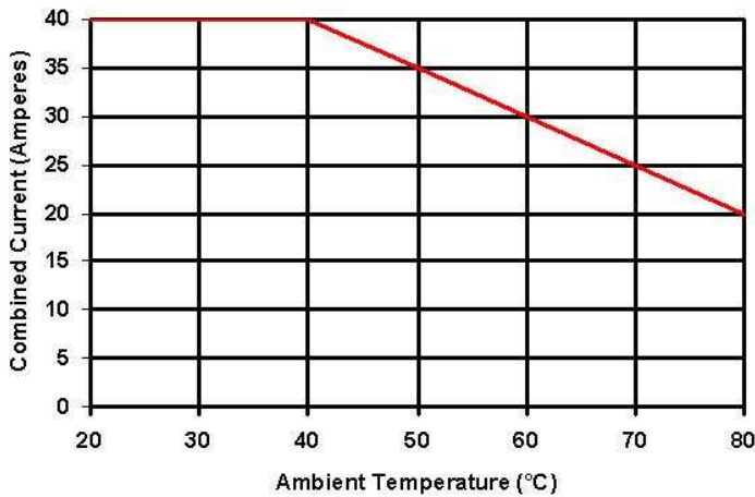
HS151DR w/50A Single or Dual SSR
