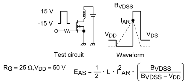
Fig. 8.16 Test Circuit/Waveform
