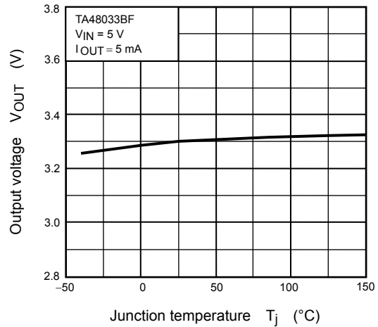
V OUT - T j
