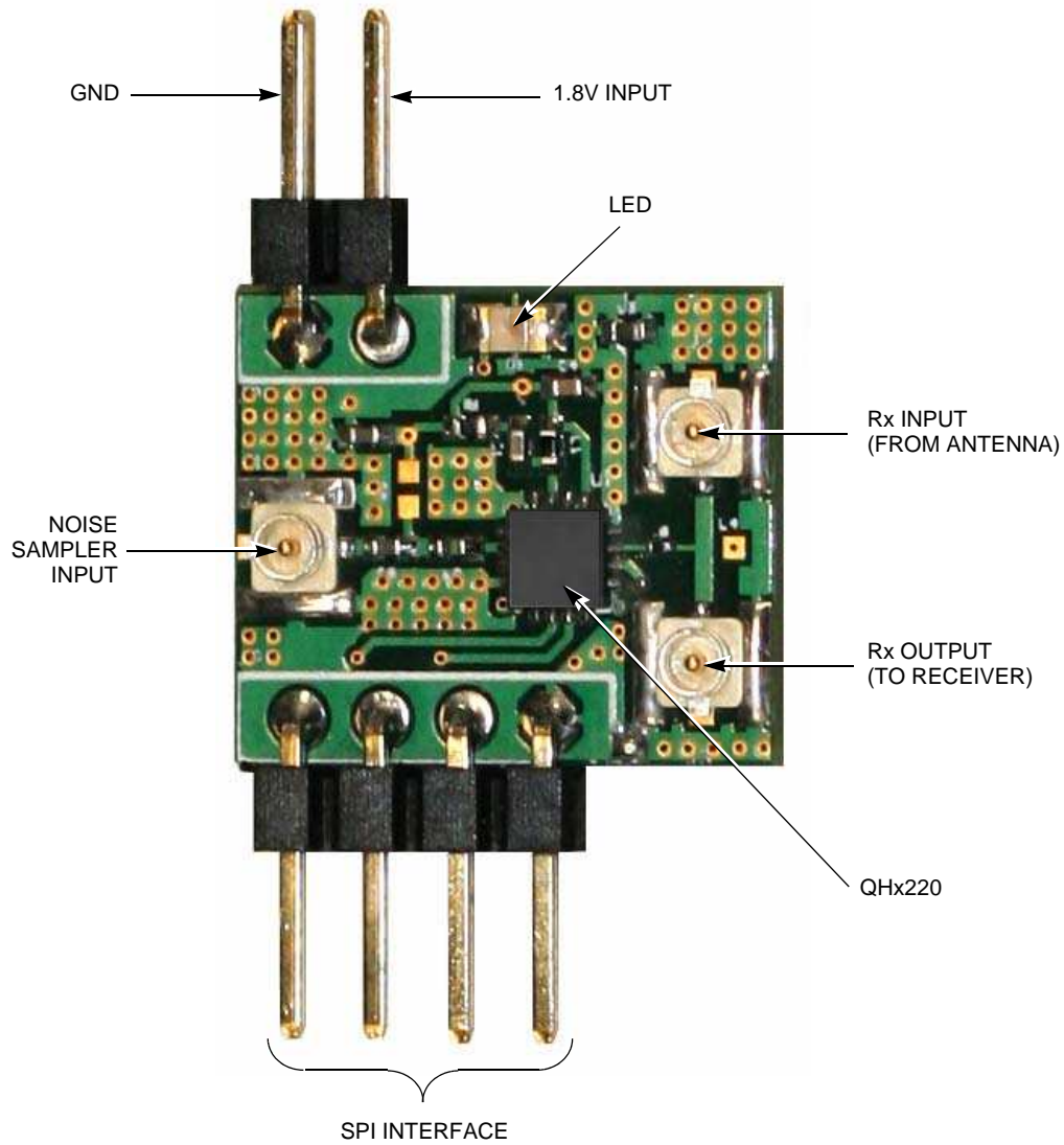
FIGURE 31. EVALUATION BOARD
