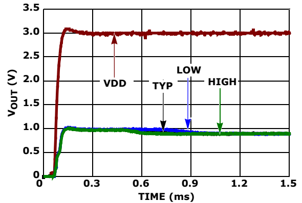
FIGURE 13. TURN-ON TIME
