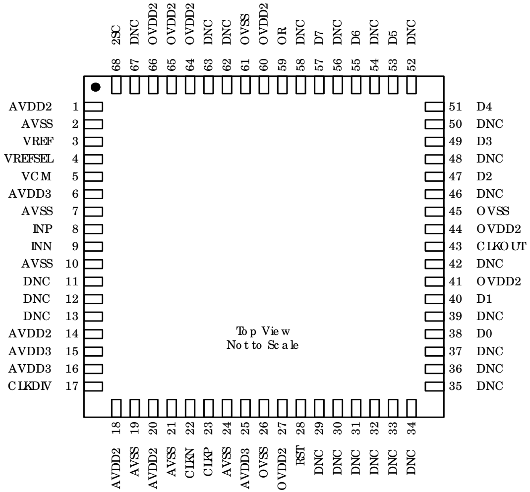
FIGURE 2. PIN CONFIGURATION
