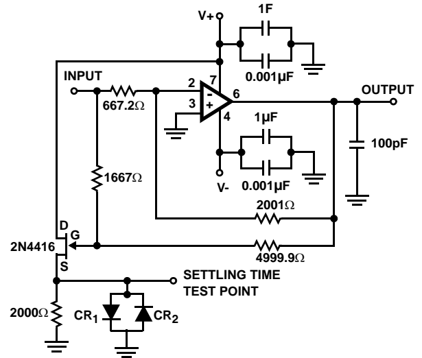
FIGURE 2. TRANSIENT RESPONSE
