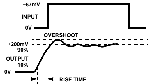
FIGURE 2. TRANSIENT RESPONSE
