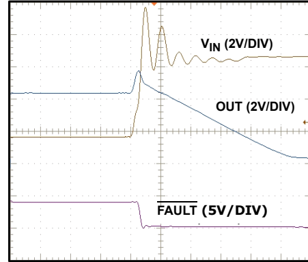
TIME - 20μs/DIV
