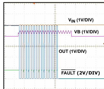
TIME - 20s/DIV
