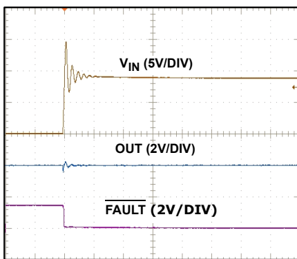
TIME - 40μs/DIV
