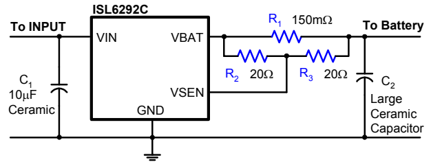
FIGURE 10. THE CIRCUIT TO GENERATE THE EQUIVALENT LOW-VALUE RESISTOR
