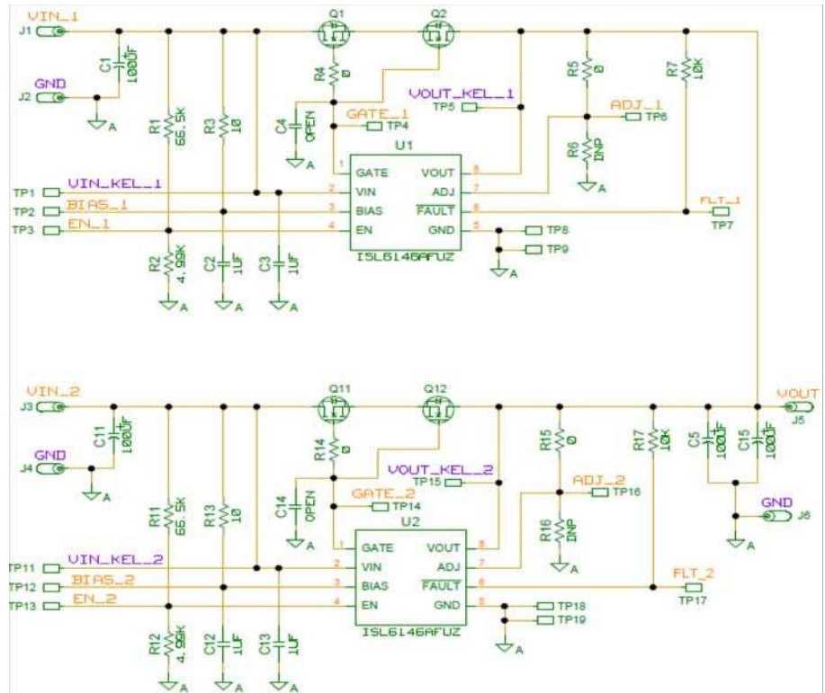
FIGURE 57. ISL6146AEVAL1Z, ISL6146DEVAL1Z SCHEMATIC
