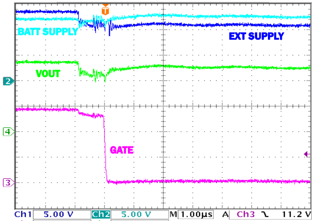
FIGURE 55. EXTERNAL SUPPLY > BATT SUPPLY DISCONNECTED
