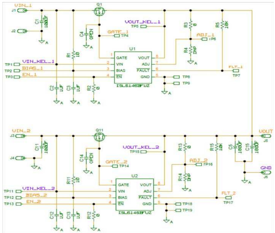
FIGURE 59. ISL6146BEVAL1Z, ISL6146EEVAL1Z SCHEMATIC
