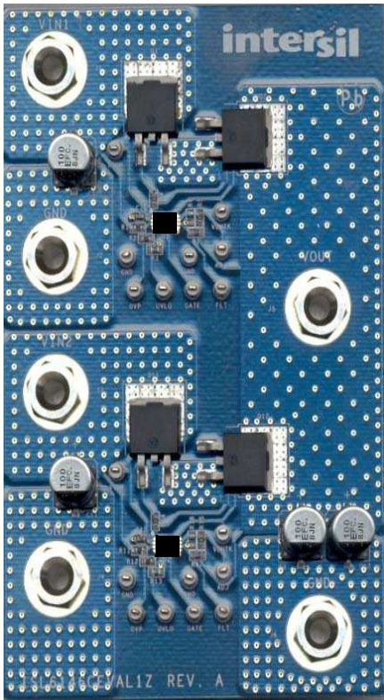
FIGURE 60. ISL6146CEVAL1Z PHOTOGRAPH
