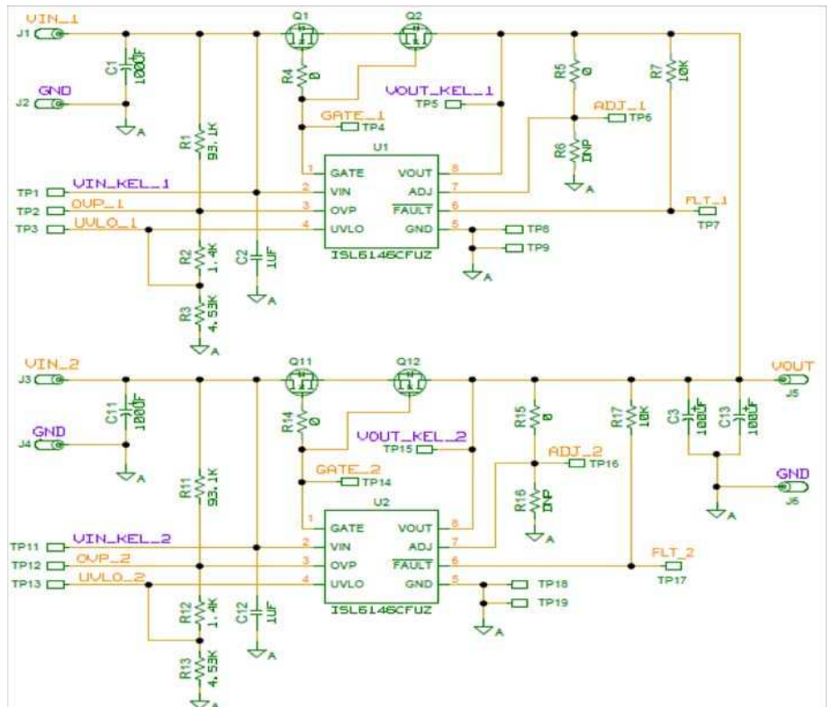
FIGURE 61. ISL6146CEVAL1Z SCHEMATIC (UVLO AND OVP TEST POINT LABELS ARE SWAPPED)
