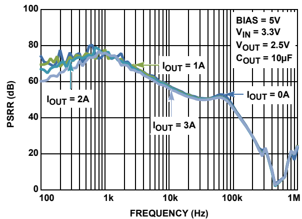
FIGURE 27. V_{IN} PSRR vs LOAD CURRENT
