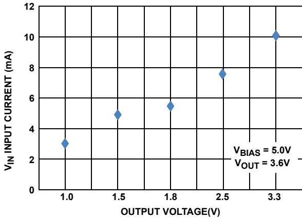
FIGURE 17. V_{IN} I_Q vs V_{OUT} VOLTAGE
