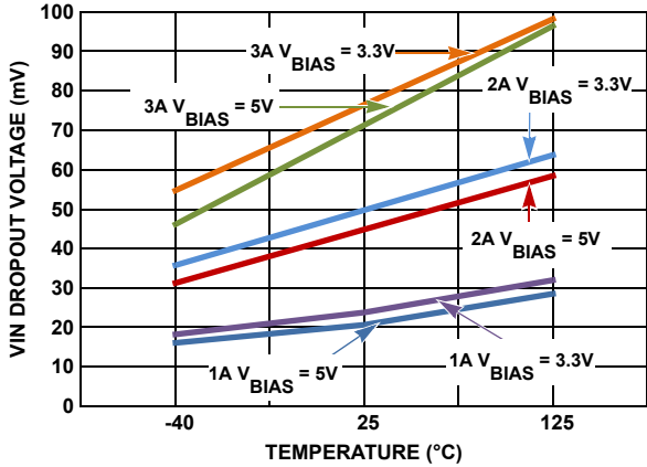
FIGURE 5. DROPOUT vs V_{BIAS}
