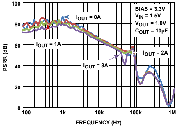
FIGURE 29. V_{IN} PSRR vs LOAD CURRENT
