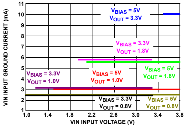
FIGURE 13. INPUT GROUND CURRENT vs V_{IN} & V_{OUT}
