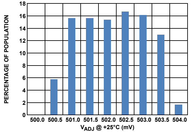
FIGURE 6. V_{ADJ} DISTRIBUTION
