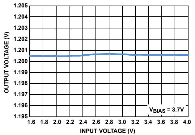
FIGURE 10. V_{IN} LINE REGULATION
