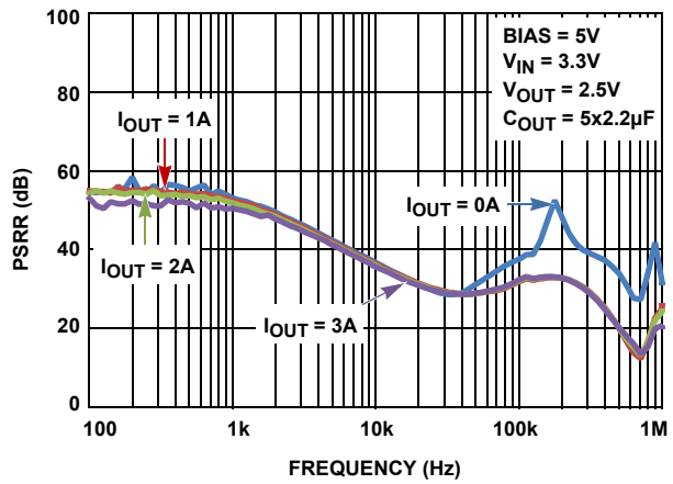
FIGURE 34. V_{BIAS} PSRR vs LOAD CURRENT
