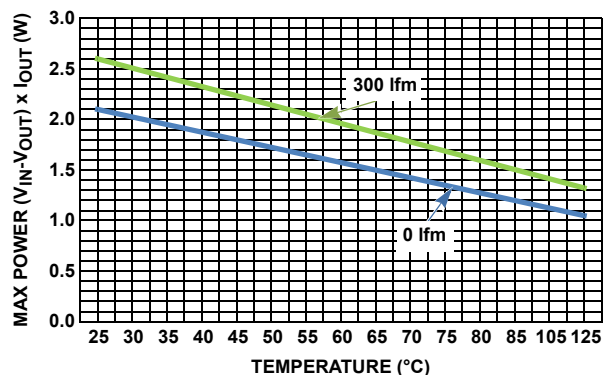
FIGURE 35. CONTINUOUS POWER LIMIT vs AIR TEMP AND FLOW
