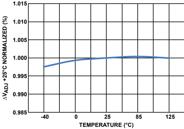
FIGURE 7. \Delta V_{ADJ} vs TEMPERATURE
