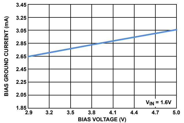
FIGURE 16. BIAS GROUND CURRENT vs V_{BIAS}
