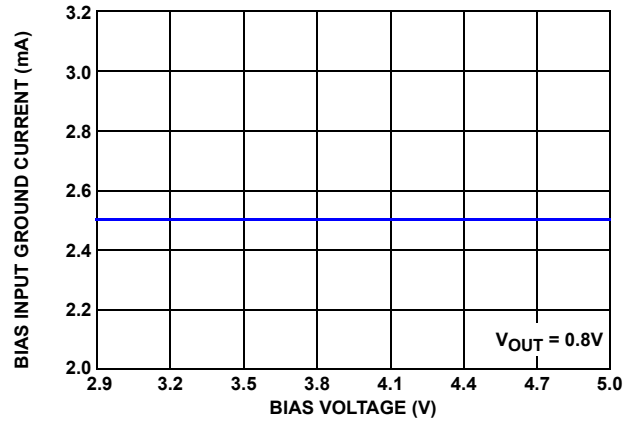
FIGURE 14. INPUT GROUND CURRENT vs V_{BIAS}
