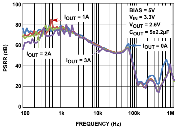
FIGURE 33. V_{IN} PSRR vs LOAD CURRENT
