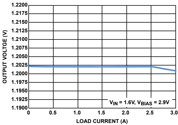
FIGURE 9. LOAD REGULATION, V_{OUT} vs I_{OUT}
