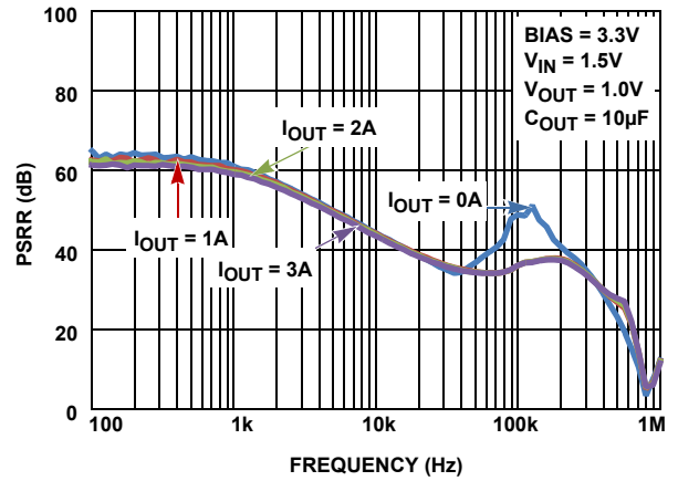
FIGURE 30. V_{BIAS} PSRR vs LOAD CURRENT
