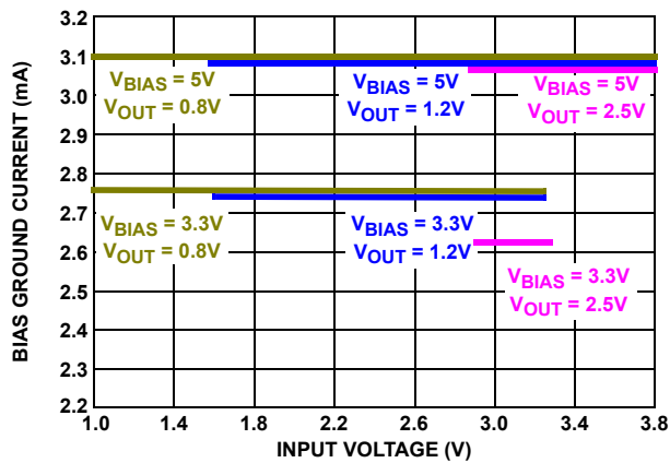
FIGURE 15. BIAS GROUND CURRENT vs V_{IN} & V_{OUT}
