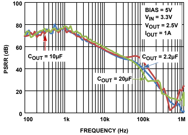
FIGURE 32. V_{IN} PSRR vs C_{OUT}
