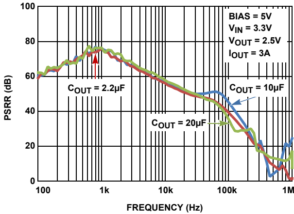
FIGURE 31. V_{IN} PSRR vs C_{OUT}
