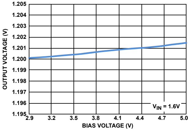
FIGURE 11. V_{BIAS} LINE REGULATION
