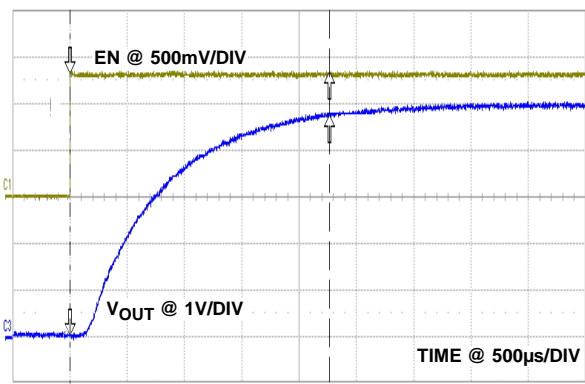
FIGURE 8. START-UP WAVEFORM
