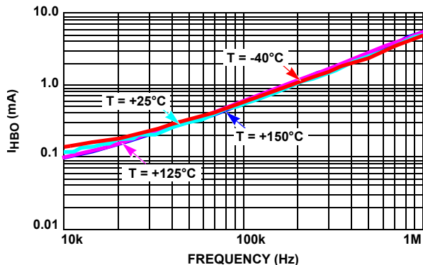
FIGURE 5. I_{HB} OPERATING CURRENT vs FREQUENCY
