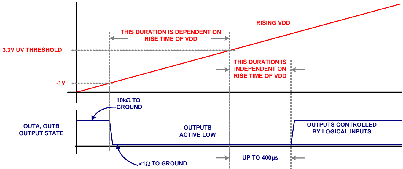
FIGURE 9. START-UP SEQUENCE
