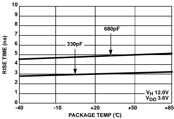
FIGURE 15. t R vs TEMPERATURE
