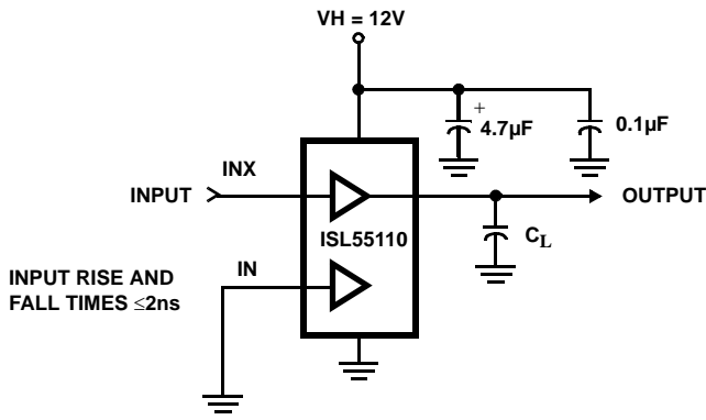
FIGURE 1. TEST CIRCUIT RISE ( t_R )/FALL( t_F ) THRESHOLDS
