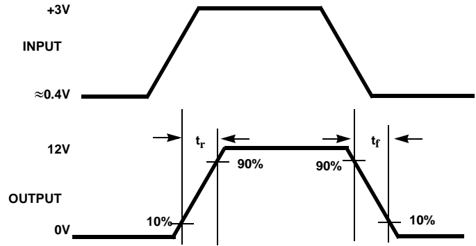
FIGURE 1. TEST CIRCUIT RISE ( t_R )/FALL( t_F ) THRESHOLDS
