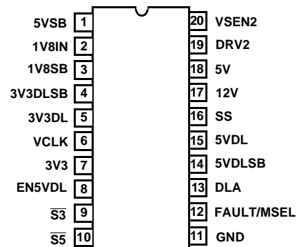
HIP6503 (SOIC) TOP VIEW
