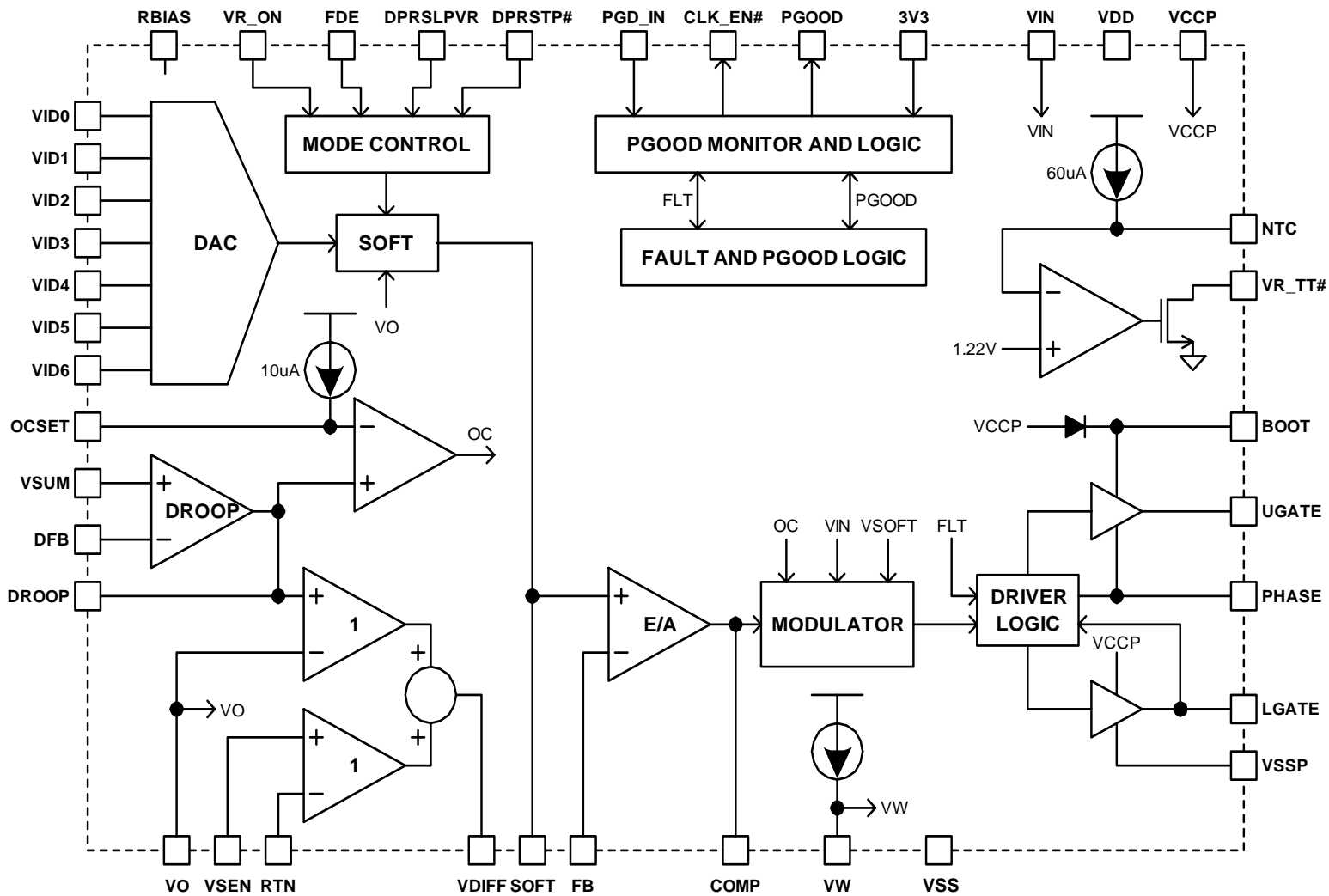
FIGURE 1. SIMPLIFIED FUNCTIONAL BLOCK DIAGRAM OF ISL6261
