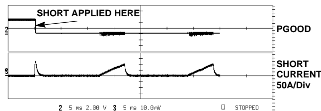
FIGURE 6. SHORT APPLIED TO SUPPLY AFTER POWER-UP
