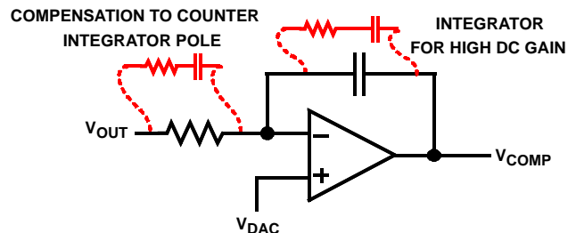
FIGURE 13. INTEGRATOR ERROR-AMPLIFIER CONFIGURATION
