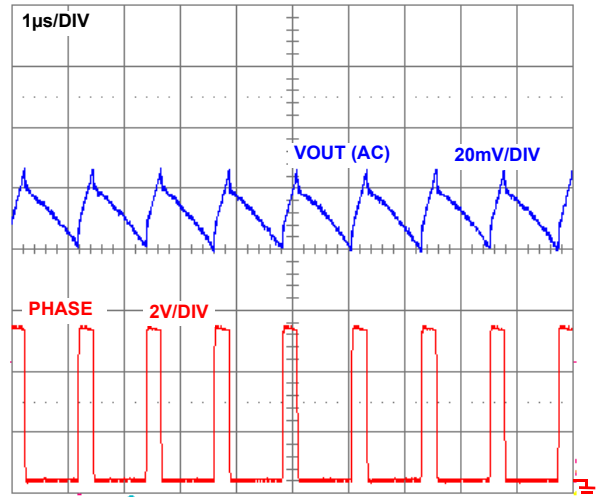
FIGURE 10. CCM STEADY-STATE
