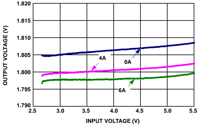
FIGURE 48. OUTPUT VOLTAGE REGULATION vs V_{IN} , T_A = +25\text{ }^\circ\text{C}
