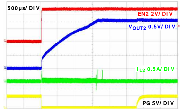
FIGURE 27. SOFT-START AT NO LOAD CHANNEL 2 (PFM)
