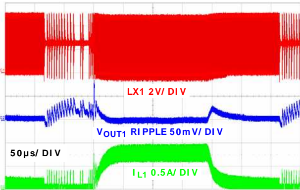
FIGURE 22. LOAD TRANSIENT CHANNEL 1 (PFM)
