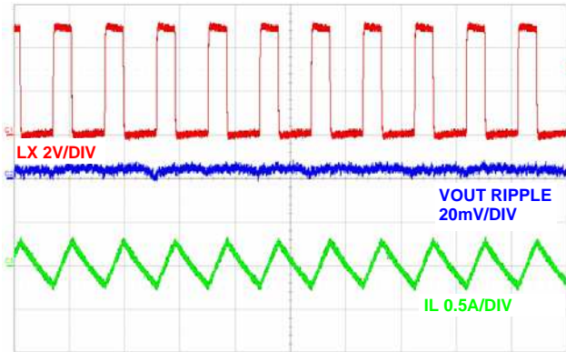
FIGURE 15. STEADY STATE OPERATION AT NO LOAD (PWM), (1µs/DIV)
