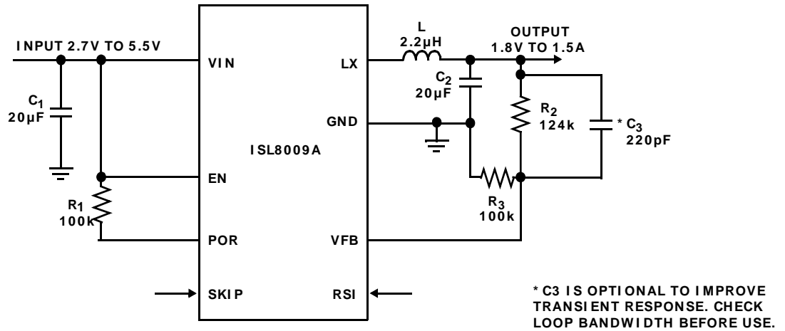
FIGURE 24. TYPICAL APPLICATION DIAGRAM
