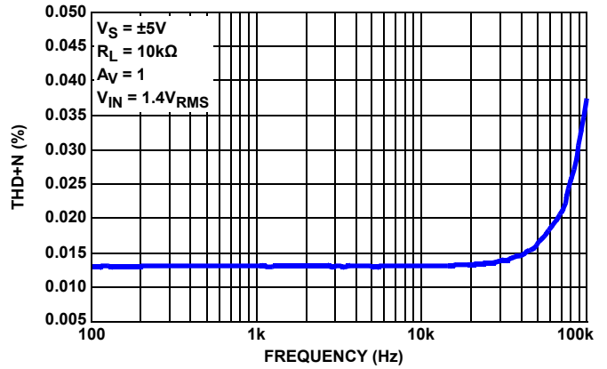
FIGURE 22. TOTAL HARMONIC DISTORTION + NOISE vs FREQUENCY
