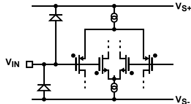
CIRCUIT 2
