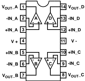
ISL28407 (14 LD SOIC, TSSOP) TOP VIEW
