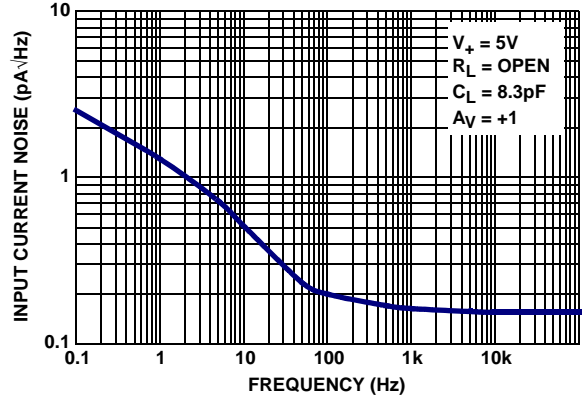
FIGURE 16. INPUT CURRENT NOISE DENSITY vs FREQUENCY
