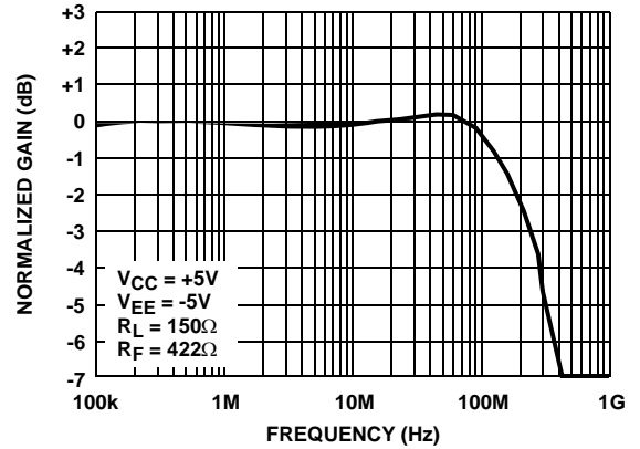
FIGURE 4. FREQUENCY RESPONSE FOR A_V = +2
