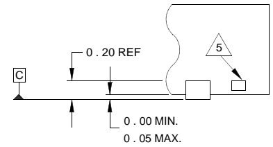
DETAIL "X"
