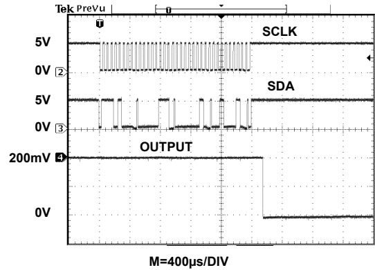
FIGURE 8. SMALL SIGNAL RESPONSE (FALLING FROM 200mV TO 0V)
