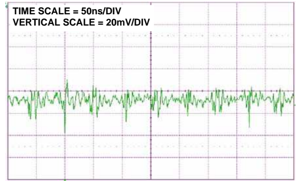
FIGURE 26. CHARGE PUMP FEEDTHROUGH AT AMPLIFIER OUTPUT
