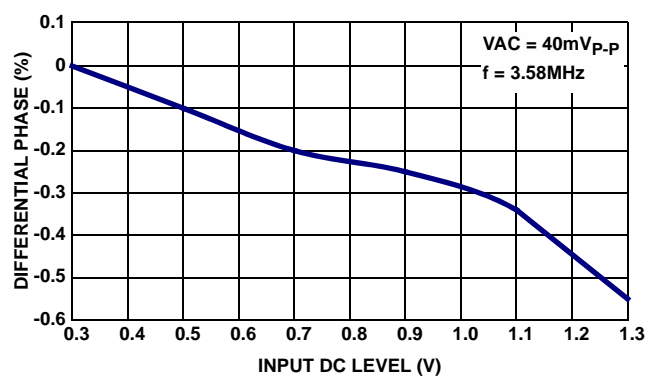
FIGURE 18. DIFFERENTIAL PHASE
