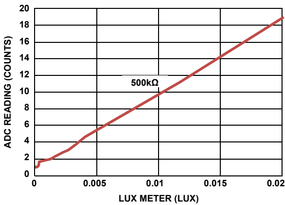
FIGURE 11. LOW LUX AT GREEN LED (500kΩ)
