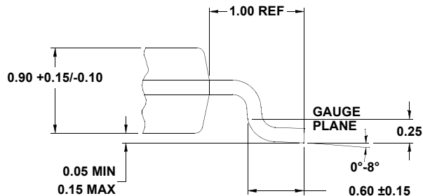
DETAIL "X"
