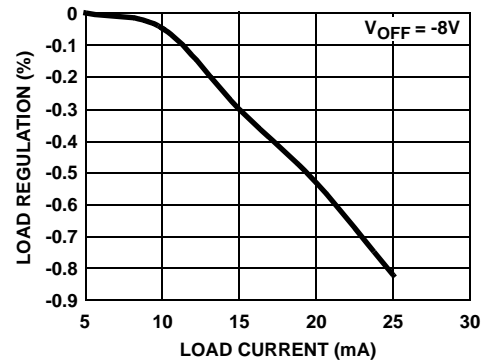
FIGURE 10. V_{\text{OFF}} LOAD REGULATION
