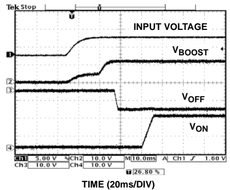
FIGURE 12. START-UP SEQUENCE
