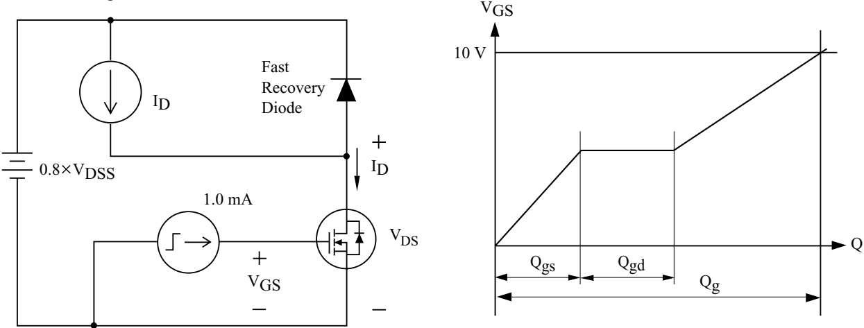
Fig14. Gate Charge
