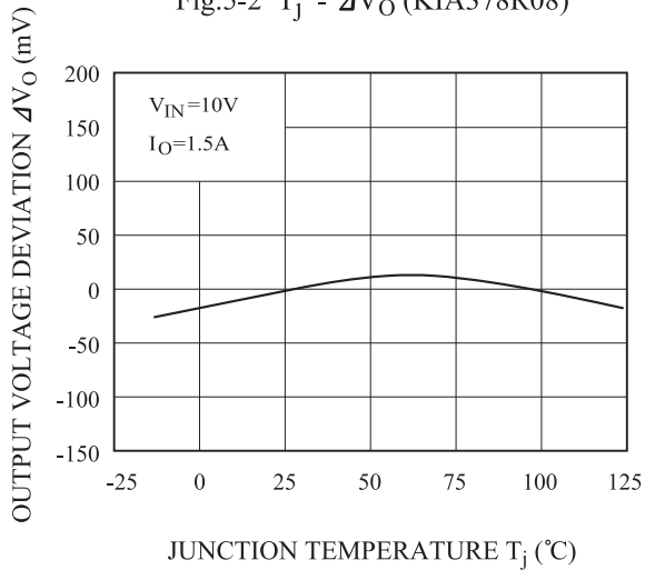
Fig.5-2 T_j - \Delta V_O (KIA378R08)
