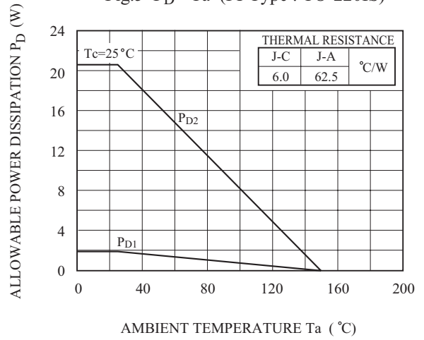
Fig.5 P_D - T_a (PI-Type : TO-220IS)
