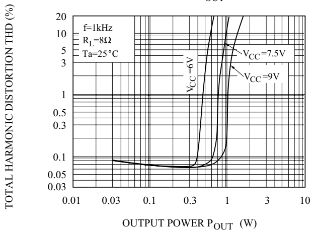
THD - P_{OUT}
