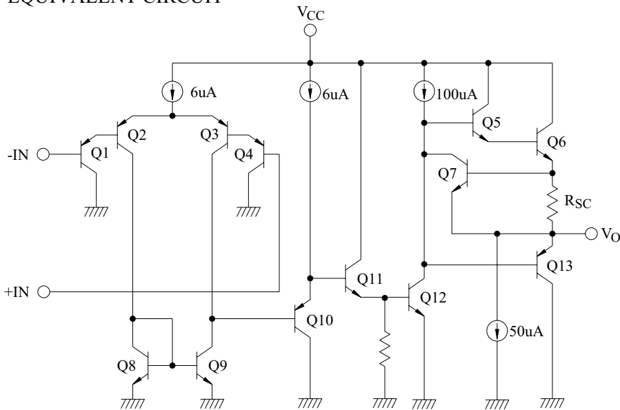
EQUIVALENT CIRCUIT
