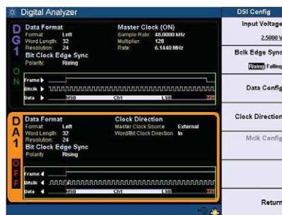
Figure 1: Configure your digital generator DSI settings, including the output format of your choice. Choose amongst four formats: PS, Left Justified, Right Justified and DSP.
