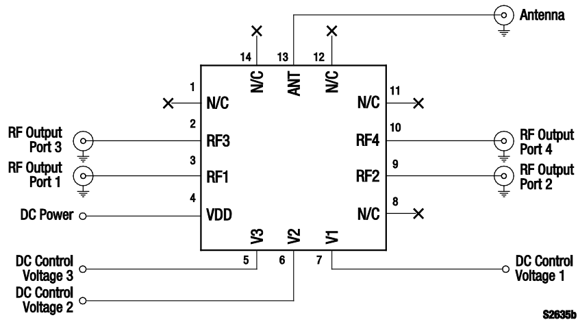
Figure 3. SKY13414-485LF Evaluation Board Schematic
