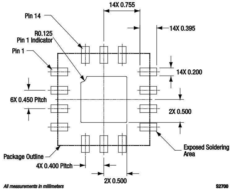
Figure 5. SKY13414-485LF PCB Layout Footprint (Top View)
