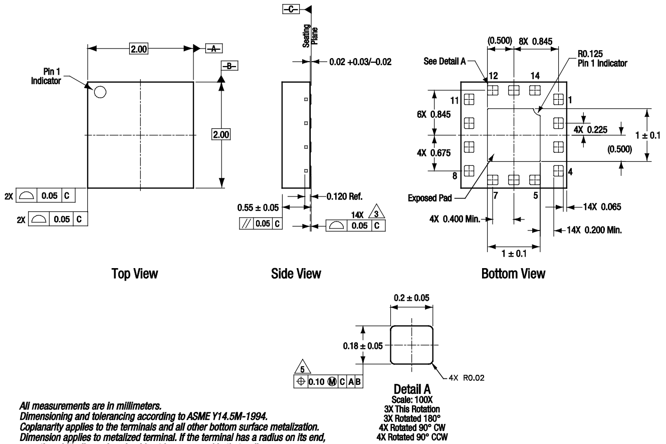
Figure 7. SKY13415-485LF 14-Pin MCM Package Dimensions
