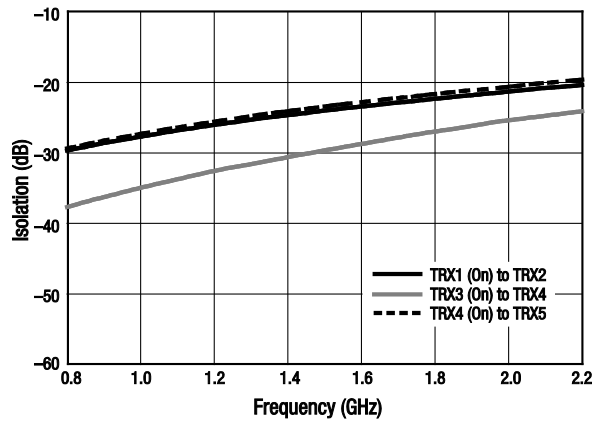
Figure 15. Isolation vs Frequency (TRX Adjacent Ports)
