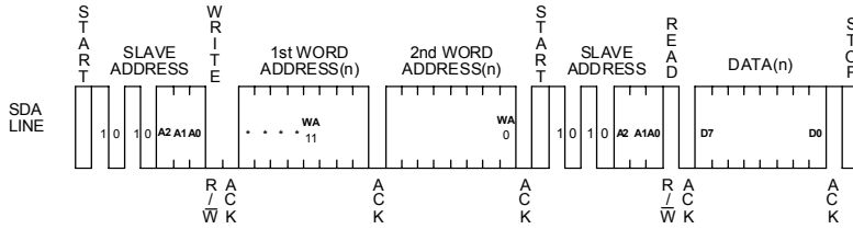
Figure 37. Random read cycle
