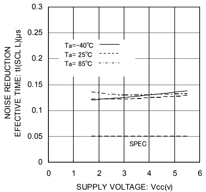
Fig. 29 Noise Spike Width t_i (SCL L)
