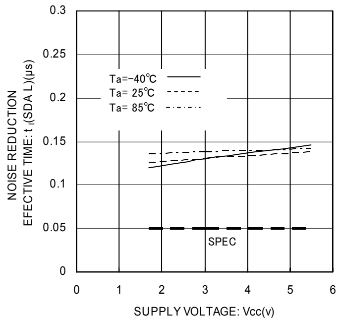
Fig. 31 Noise Spike Width t_i (SDA L)
