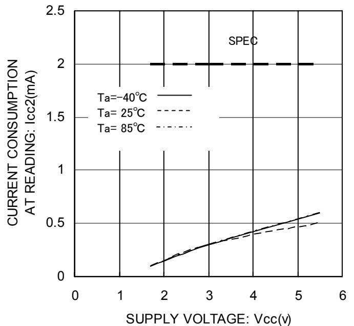
Fig.11 Current consumption at READ operation I_{cc2} ( f_{scl}=1MHz )
