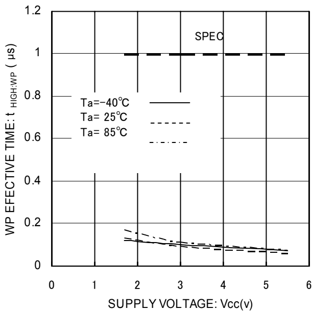
Fig. 34 WP High Time t_{HIGH:WP}
