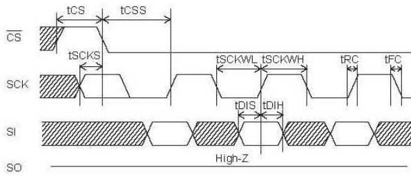
Figure 1. Input timing
