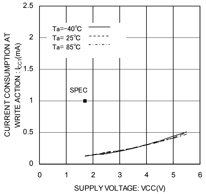
Figure 13. Current consumption at WRITE action I_{CC1}(WRITE, f_{SK}=1MHz)
