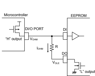
Figure 53. Circuit at DI, DO direct connection (Microcontroller DI/O "H" output, EEPROM "L" output)
